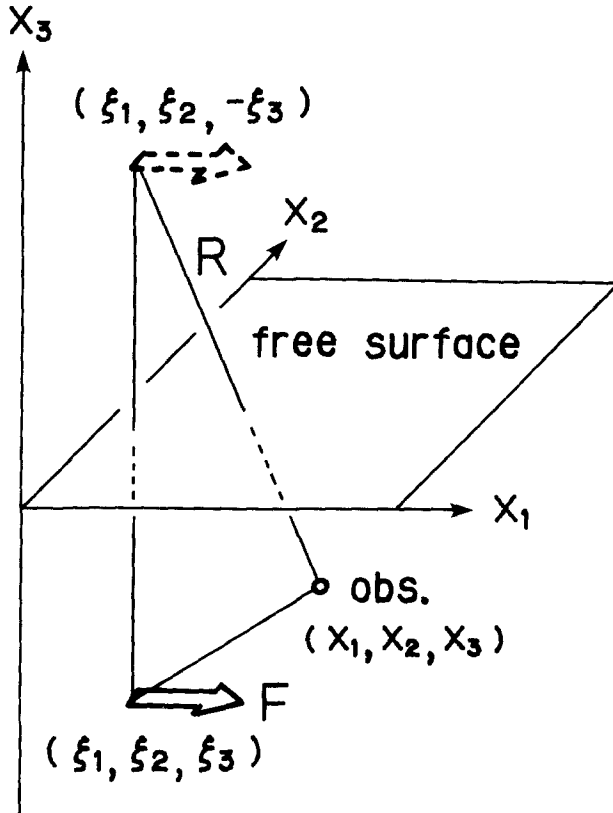
FIG. 1. A coordinate system adopted in this study.
