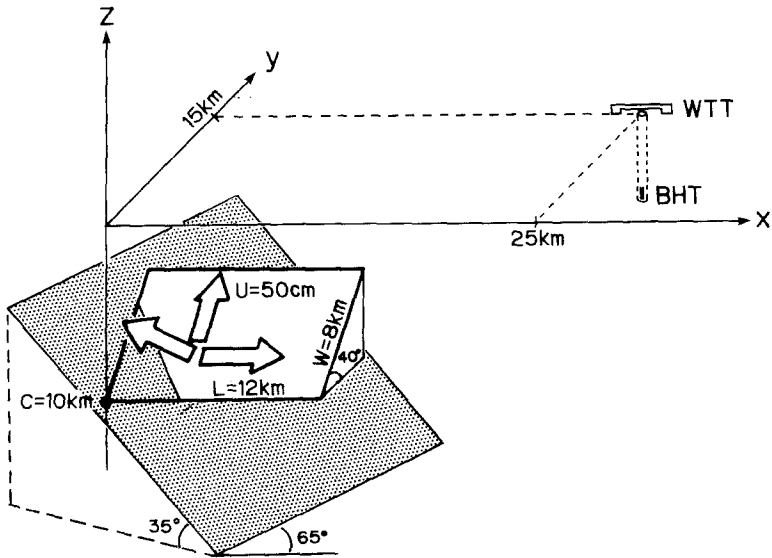
FIG. 8. An example of the tilt observations at ground surface and in a borehole. Note that a water-tube tiltmeter (WTT) measures \partial u_z / \partial x , while a borehole tiltmeter (BHT) measures \partial u_x / \partial z . A shaded oblique plane crossing the fault surface corresponds to the observation plane in Figure 6.
